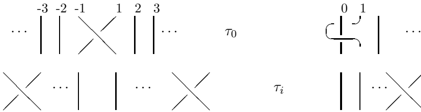
Figure 1: The graphical interpretation of the generators as symmetric tangles (on the left) and as cylinder tangles (on the right)
