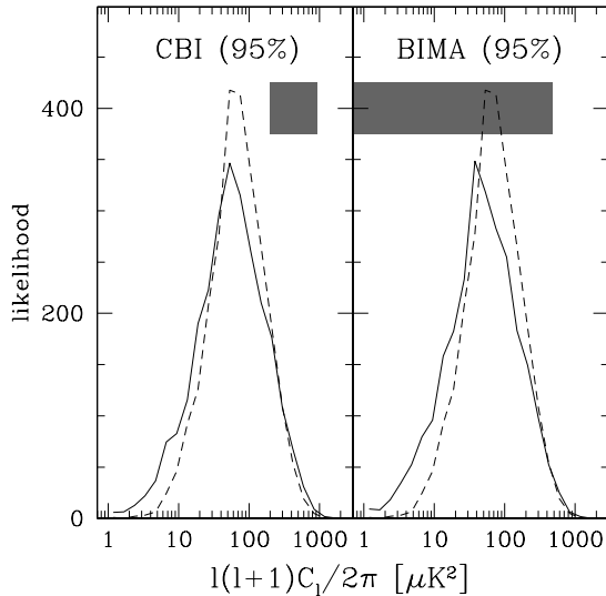
FIG. 1.— Unnormalized probability distribution of the SZ angular power spectrum in CBI (left panel) and BIMA (right panel) high- l averaged windows (solid lines), weighted by the primary CMB likelihood. The gray areas show 95% confidence regions of the CBI (Mason et al. 2002) and BIMA (Dawson et al. 2002) data, assuming Gaussian fluctuations. Note that the true error is larger because of non-Gaussian nature of the SZ fluctuations, and depends on cosmological models. Also shown is the result using analytic approximation of Komatsu and Seljak (2002) for C_l (dashed lines).
