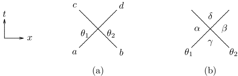
Fig. 1: (a) The 2-particle scattering process a(\theta_1) + b(\theta_2) \rightarrow c(\theta_2) + d(\theta_1) (b) The 2-kink process K_{\alpha\gamma}(\theta_1) + K_{\gamma\beta}(\theta_2) \rightarrow K_{\alpha\delta}(\theta_2) + K_{\delta\beta}(\theta_1)
